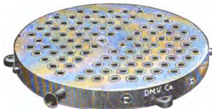
FIG. 213.—One-piece Cast Burner Body of the Dayton Burner.
